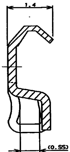
SECT "D" - "D" (SCALE 20-1)
