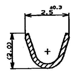
SECT "B" - "B"
